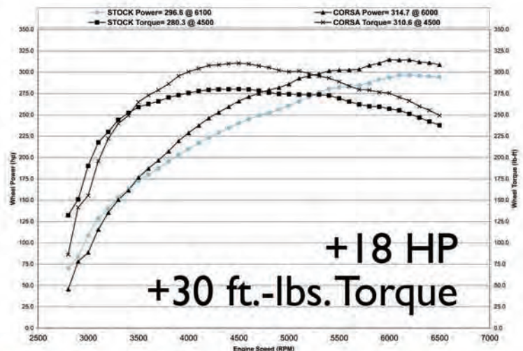
2006 CHEVROLET TRAILBLAZER SS 6.0L V8 - CHASSIS DYNO TESTING SAE Standard Corrected Data; Average Data of 3 Runs Each
