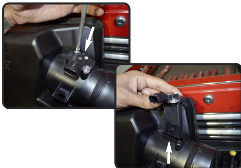
9. Loosen the 2 screws holding in the MAF sensor. Now lift up the MAF sensor and remove.
