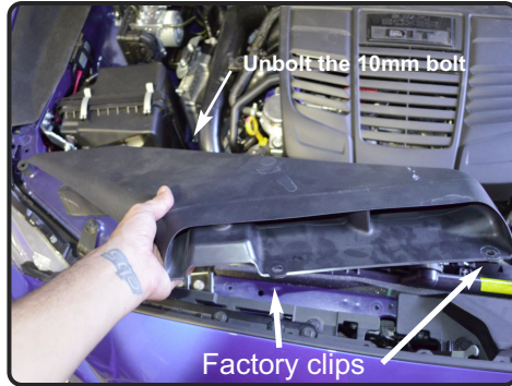
2. Remove the two plastic retaining rivets from the air scoop and remove scoop from engine bay. Save for later install. Loosen the 10mm bolt holding in the lower part of the air box to the vehicle frame.
