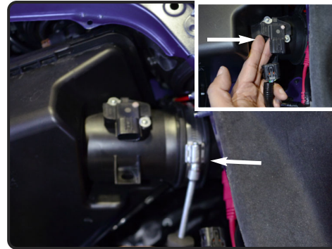
4. Disconnect the MAF sensor harness. Loosen the clamp on the airbox using 8mm nut driver. un-clip air box. remove lower half first. Now remove the upper half and remove. The complete air box assembly should be removed.
