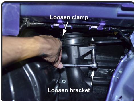
5. Loosen the clamp on the turbo intake tube. With 10mm socket, loosen the bracket on intake tube from OEM vibramount. loosen the backside of the vibramount.
