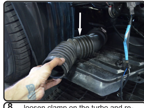
8. loosen clamp on the turbo and remove the lower intake tube.
