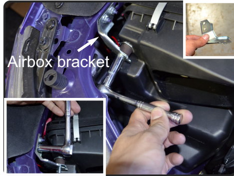
3. With 10mm socket and ratchet, loosen the nut holding in the airbox bracket. Loosen the 2 nuts holding in the airbox bracket and remove. Save air box bracket and oem isolation mount for later install.
