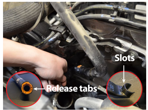
15. Line up the slots on the Injen release tool to the crank case fitting slots and then firmly pull the line. This will unlock the tabs required to release the fitting.
