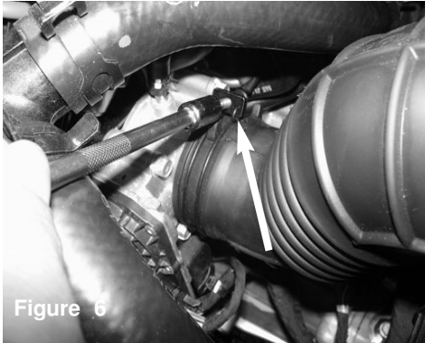
Figure 6 Use a 10mm socket/ratchet to loosen the clamp in the throttle body.
