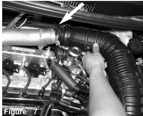
Figure 7 Use a 10mm socket and ratchet and loosen the 10mm clamp bolt on the air duct located on the Turbo charger compressor outlet. Pull the air duct from the outlet.
