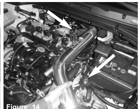
Figure 14 Position the intake pipe into the engine bay and place the end of the pipe into the step hose on the turbo compressor outlet.
