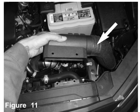
Figure 11 Re-install the ram scoop from step 4 and secure.
