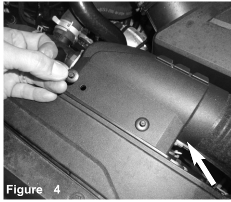
Figure 4 Remove the 2 push clips from OEM air box. Remove the ram scoop. Save for later install.
