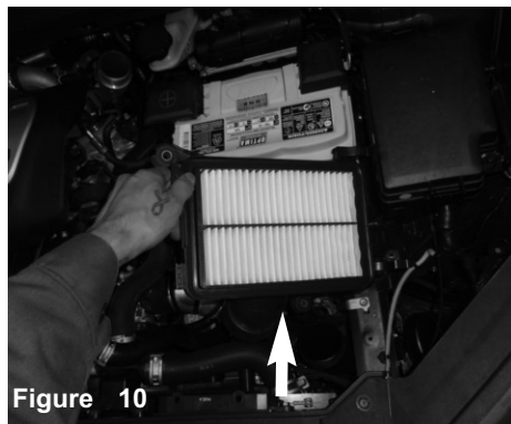
Figure 10 Now the lower air box assembly can be removed from the engine bay.
