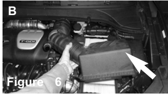
Figure 6 Figure A: Unclip the two tabs from the lower air box assembly to the upper air box assembly. Figure B: Detach the upper air box assembly from the lower assembly
