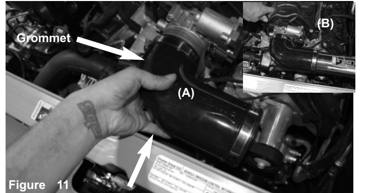
Install the elbow with clamps provided to the throttle body. Make sure the short side with grommet is on the throttle body. (A) (B)
