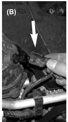
Figure 4 (A) Stock air temp sensor on factory air duct. Figure 4 (B) Unclip harness from from air temp sensor.
