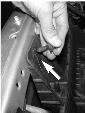
Figure 8 (A) Loosen the bolt holding in the air box plastic bracket closes to the headlight. Figure 8 (B) Remove the bolt and save for the bracket install.
