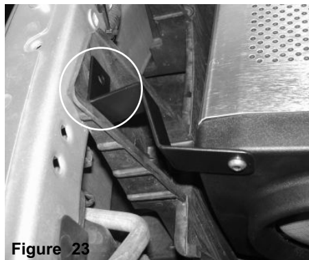
Figure 23 Position the bracket to the hole from step 8. Secure the bracket using factory screw.
