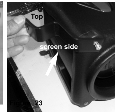
Figure 23 Now install the bracket p/n:20108 to the front of the powerflow box.
