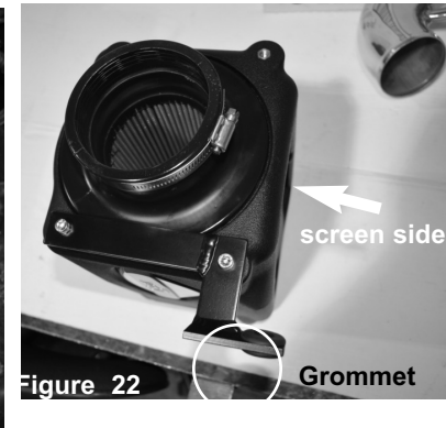
Figure 22 Install the bracket p/n:x-20109 to the power-flow box. Make sure its install to the back side of the power flow box. Install grommet to the bracket hole.
