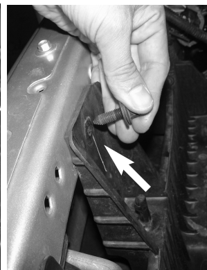
Figure 8 (A) Loosen the bolt holding in the air box plastic bracket closes to the headlight. Figure 8 (B) Remove the bolt and save for the bracket install.
