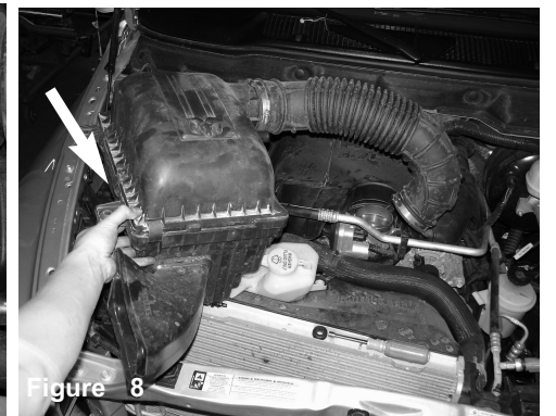
Figure 8 Lift factory air box cleaner and pull entire air box and air duct assembly out of engine bay.
