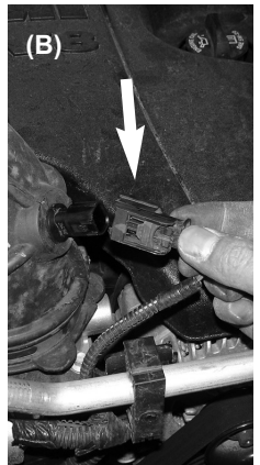
Figure 4 (A) Stock air temp sensor on factory air duct. Figure 4 (B) Unclip harness from from air temp sensor.
