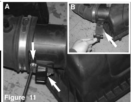
Figure 11 Figure A: Use a Torx driver to remove the two screws from the MAF sensor located on the upper air box assembly. Figure B: Remove the MAF sensor from the upper air box housing.
