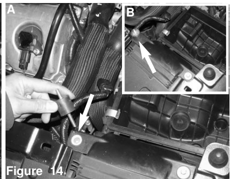
Figure 14 Figure A: Place the long ended stud of the vibra mount into the same hole the 10mm bolt was removed from. Figure B: Vibra mount shown mounted in place.
