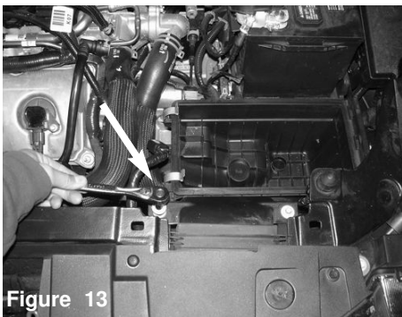
Figure 13 With the air scoop cover removed, you may now remove the left 10mm air scoop bolt
