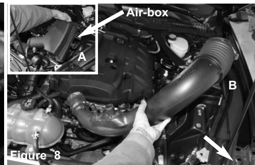
Figure 8 A) Lift up and remove the air box out of the vehicle. B) Now remove the intake tube out of vehicle.
