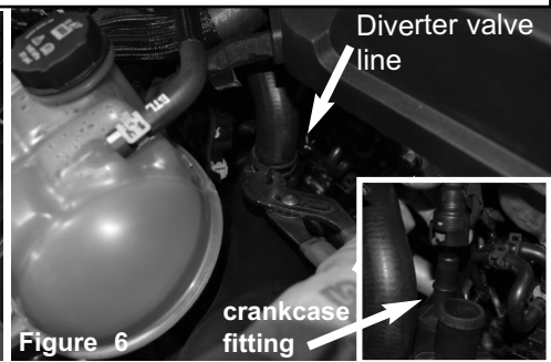
Figure 6 On the intake tube near turbo, loosen the clamp on the diverter valve line. Pull line away from tube. Disconnect the crankcase line on tube also.
