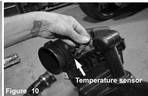
Figure 10 Remove the temperature sensor out of the airbox. Turn and pull the temperature sensor out of tube.
