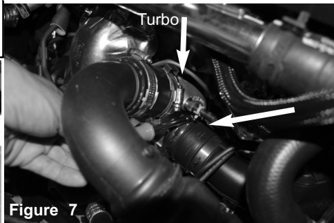
Figure 7 On the end of the intake tube, loosen the clamp on the turbo.
