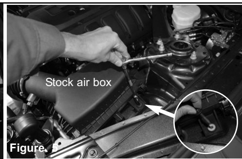
Figure 5 Locate the screw holding in the air box. Loosen using 10mm nut driver or socket. Remove the screw.
