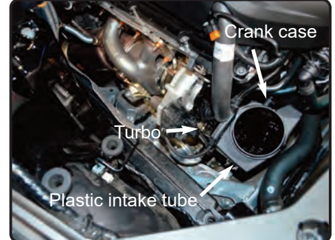
8. Re-install the plastic intake tube into the vehicle. Re-connect Crank case line. Make sure you hear a click, tug on tube to make sure the tube is secured to turbo and will not come off.
