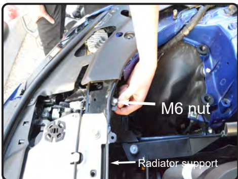
14. Make sure the heatshield is flat on frame. Locate the hole on the radiator support.
