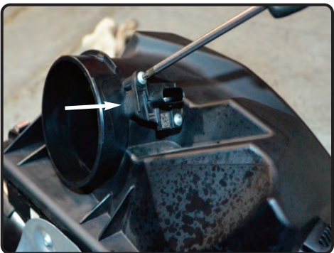
18. Loosen the 2 screws holding in the temp sensor using T25 torx bit and remove from air box.
