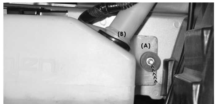
Align the three holes in the reservoir tank to the three pre-tapped holes located in the car frame. Screw the long stud on the vibra-mount over the reservoir tank and into the pre-tapped hole until the tank is firmly fastened(A). Firmly press the end of the spout into the grommet until a proper seal has been achieved(B).
