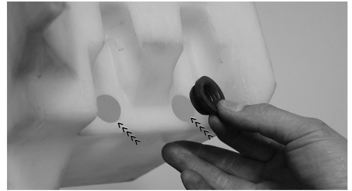
Remove the stock motor grommets from the stock reservoir tank. Press the two stock grommets into the pre-drilled 21mm holes in the new reservoir bottles.
