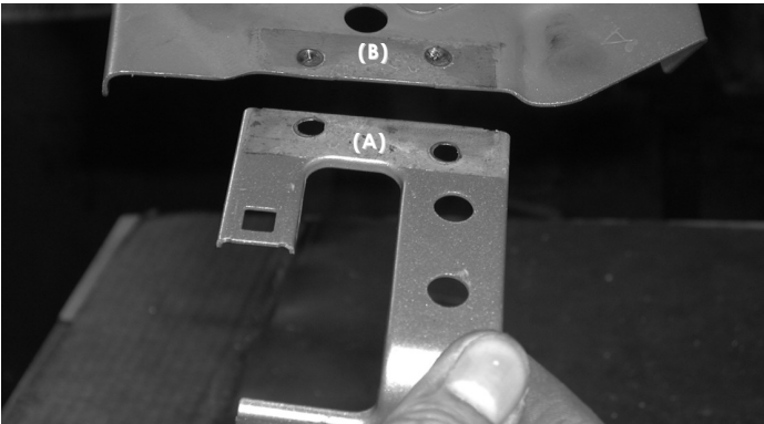
Once the bracket on the battery tray is broken loose(A) go ahead and reinstall the battery tray back to its stock location (B).
