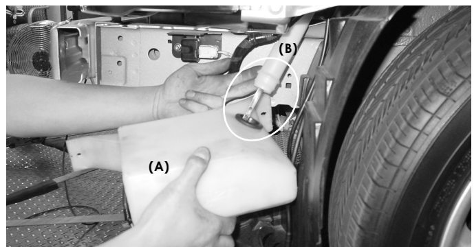
Position the new reservoir tank in the same stock location (A). Press the bottom end of the stock spout into the large grommet on the tank(B).
