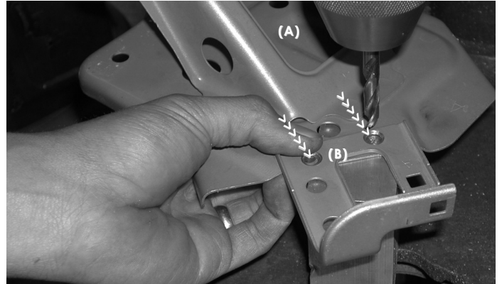
The battery tray is removed from the RSX (A). Turn the battery tray upside down and drill the two tacked or spot welded areas until the bracket becomes loose (B).
