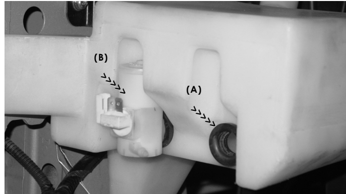
Once the stock grommets have been pressed into the pre-drilled holes(A) take the stock motors and press them into the stock grommets(B).
