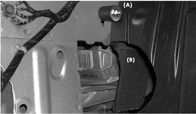
This is the location of the vibra-mount prior to setting the reservoir tank in place. The tank is placed under the vibra-mount, this is for demonstration of the location only (A). The opening that leads into the engine compartment when installing the intake(B).
