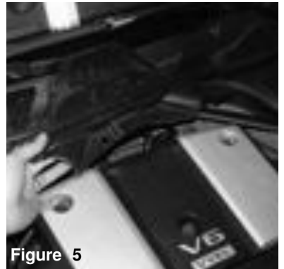
Figure 5 The stabilizer bar cover is now removed.
