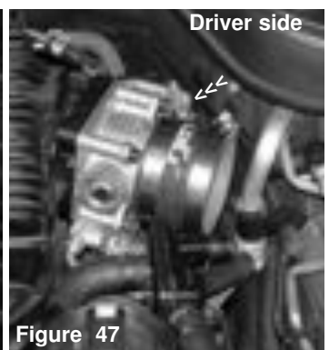
Press the 2 3/4" straight hose over the throttle body until it sits flush up against the base. Place two power-clamps over the straight hose and tighten the clamp on the throttle body side.
