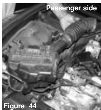
With the harness and bolt out of the way, continue to pull the entire air box cleaner and air intake duct from the engine compartment.
