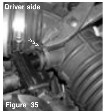
Using a pair of needle nose pliers or regular pliers, compress the tension clamp on the crankcase ventilation box and pull the CCV box out from the air intake port.
