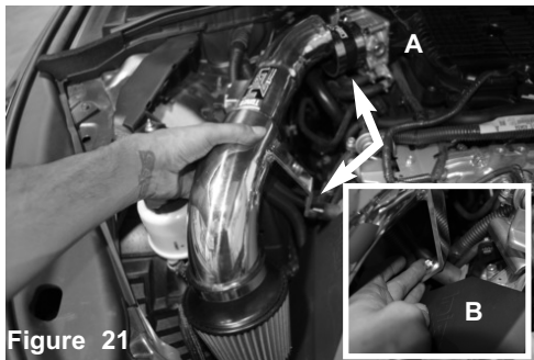
A) Install passenger side intake tube assembly. B) Secure the bracket to the vibramount from step 13 using provided M6 nut and fender washer.
