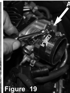
A) Install driver side intake tube assembly. B) Secure the bracket to the vibramount from step 14/15 using provided M6 nut and fender washer. C) Connect the crank case box to the fitting using provided 17mm hose. Make sure the plastic fitting goes inside the fitting welded on tube.
