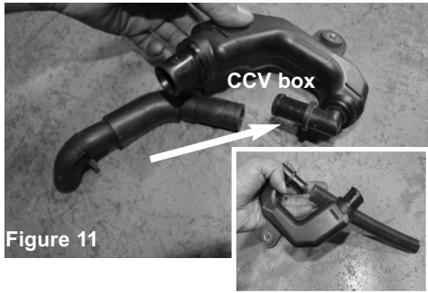
With pliers, remove the factory hose from the fitting on CCV box. Replace with new provided 15mm hose to the same fitting.
