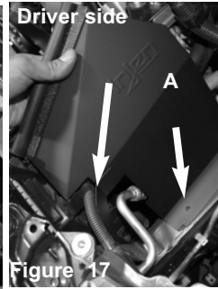
A) For both the passenger and driver side, remove the MAF sensors using 7mm nut driver. B) Install MAF sensors into the new intake tubes and secure using the OEM screws.
