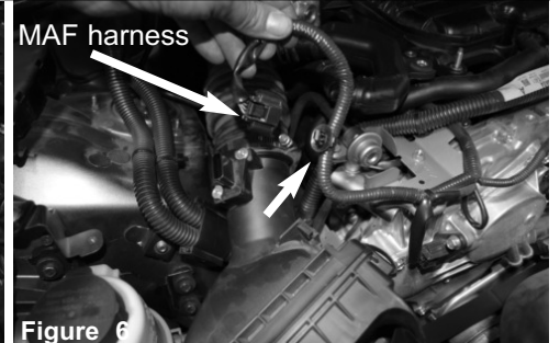
Figure 6: For both Driver and Passenger side, disconnect the MAF sensor harness and pull harness clip away from airbox.
