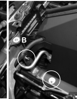
A) For both the passenger and driver side, remove the MAF sensors using 7mm nut driver. B) Install MAF sensors into the new intake tubes and secure using the OEM screws.
