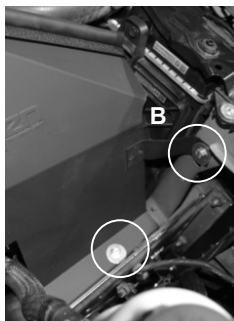
A) Install the passenger side heatshield to the vehicle and position the bracket to the threaded holes on the vehicles frame. Note: Bracket is between plastic hardline and a/c line. Attach Rubber trim seal to the top of the heat shield. B) Secure the heatshield using provided M6 hex screws and washers. Tighten and secure using 10mm socket and ratchet.
