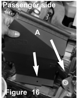
A) Install the passenger side heatshield to the vehicle and position the bracket to the threaded holes on the vehicles frame. Note: Bracket is between plastic hardline and a/c line. Attach Rubber trim seal to the top of the heat shield. B) Secure the heatshield using provided M6 hex screws and washers. Tighten and secure using 10mm socket and ratchet.
