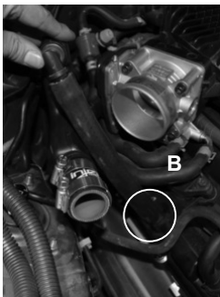
A) Now install the 1-1/8" hose with mini clamps provided to the fitting on larger side. B) Now install the new CCV assembly to fitting on engine. Position like above image. Push CCV box behind Throttle body.
