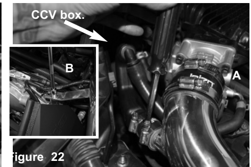
A) Position the crank case assembly from steps 10-12 to the large fitting on tube. Position for the CCV box to fit and not touch anything. B) Tighten both passenger and driver side brackets using 10mm socket and ratchet. Tighten the clamps using 8mm nut driver on throttle body.
