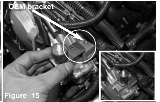
Now install the bracket extension assembly to the insert from the previous step. Make sure the offset hole is in the correct position. Secure and tighten the bracket using the original screw using 10mm socket or wrench.
