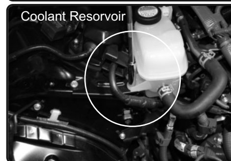
11. Locate the coolant reservoir screw, loosen this bolt and save for later install.
