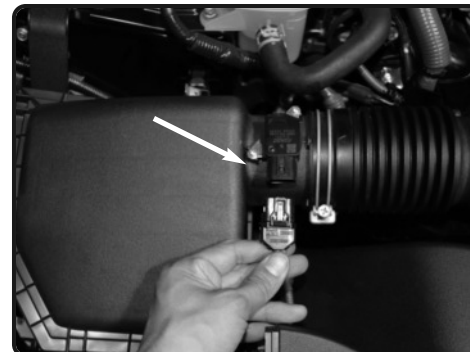
3. Disconnect the MAF sensor harness.
