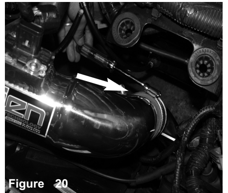
Figure 20 Position best possible fit and tighten remaining clamps using 8mm nut driver.
